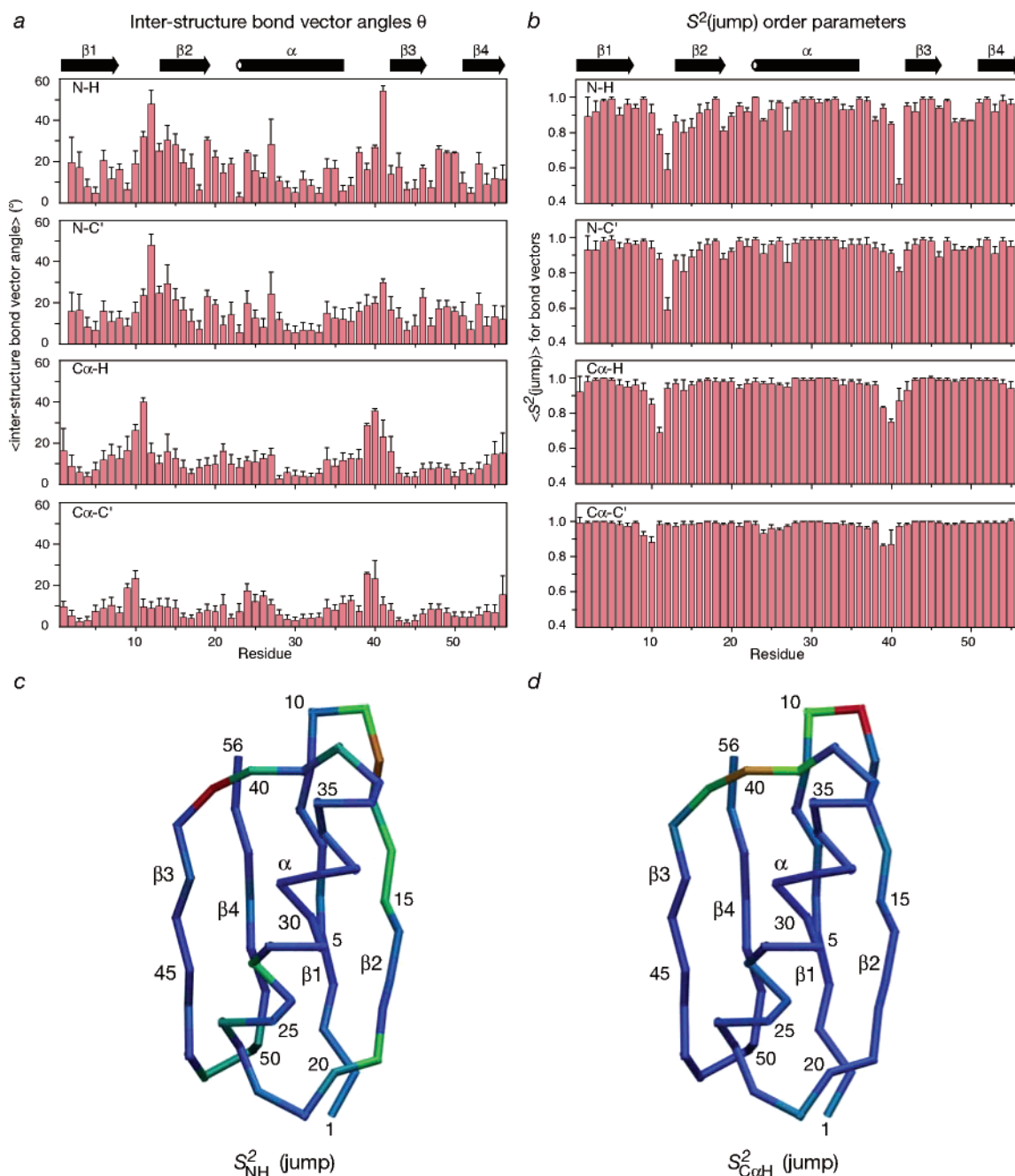
FIGURE 2: Amplitudes of backbone motions for GB3 deduced from the ensemble size N_e = 2 structures. The average interstructure N-H, N-C', Cα-Hα, and Cα-C' bond vector angles, \langle \theta \rangle , between members of an ensemble and the corresponding calculated average order parameters, \langle S^2(\text{jump}) \rangle (where the angle brackets denote averaging over all 100 calculated ensembles), are displayed as a function of residue in panels a and b, respectively. The error bars are the standard deviations from the 100 calculated ensembles. The secondary structure elements are shown above the figure: strands β1, β2, β3, and β4 comprise residues 1–8, 13–20, 42–46, and 51–56, respectively; the single α-helix extends from residue 23 to residue 36. Panels c and d display a Cα backbone trace of the GB3 domain color coded according to \langle S^2(\text{jump}) \rangle for the N-H and Cα-Hα bond vectors, respectively. The values of \langle S^2(\text{jump}) \rangle vary linearly through the color spectrum from red to blue, corresponding to the minimum and maximum values of \langle S^2(\text{jump}) \rangle , respectively.
